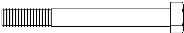
3/8-16 X 3.5" HEX HEAD BOLT X20 F0001
