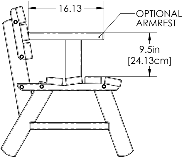
3 BENCH WITH ARMREST DETAILS
