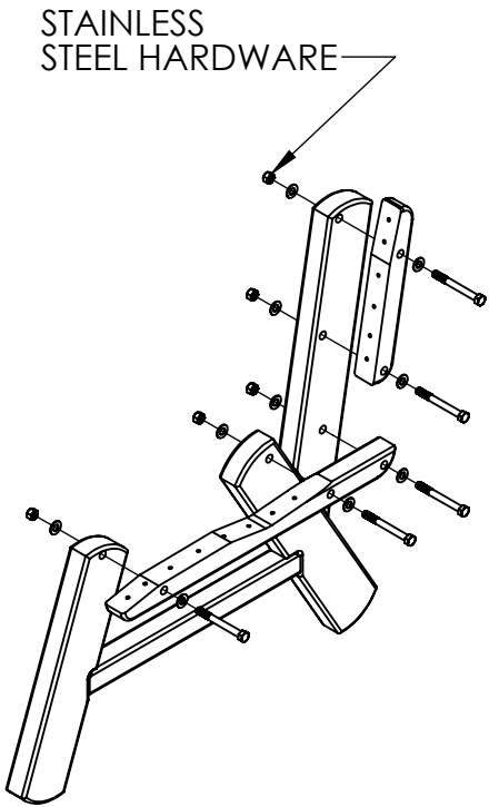
2 HARDWARE DETAILS
