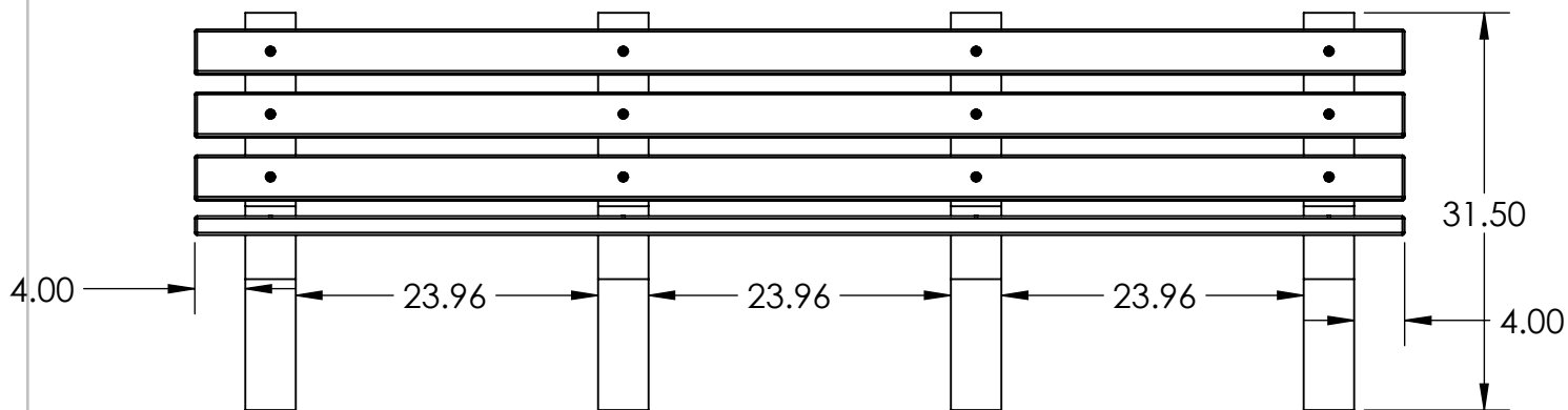
FRONT VIEW
